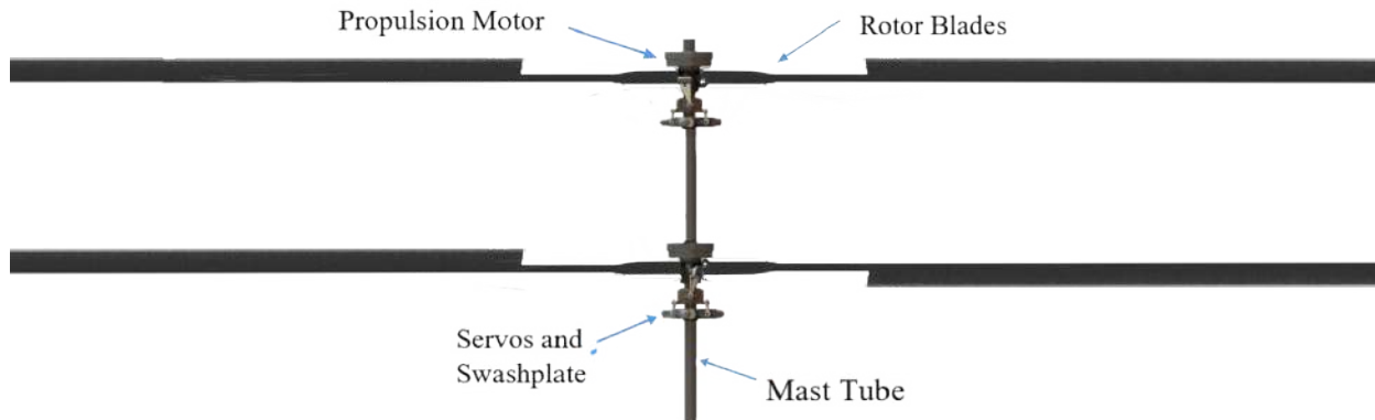
Figure 10: Propeller Configuration
