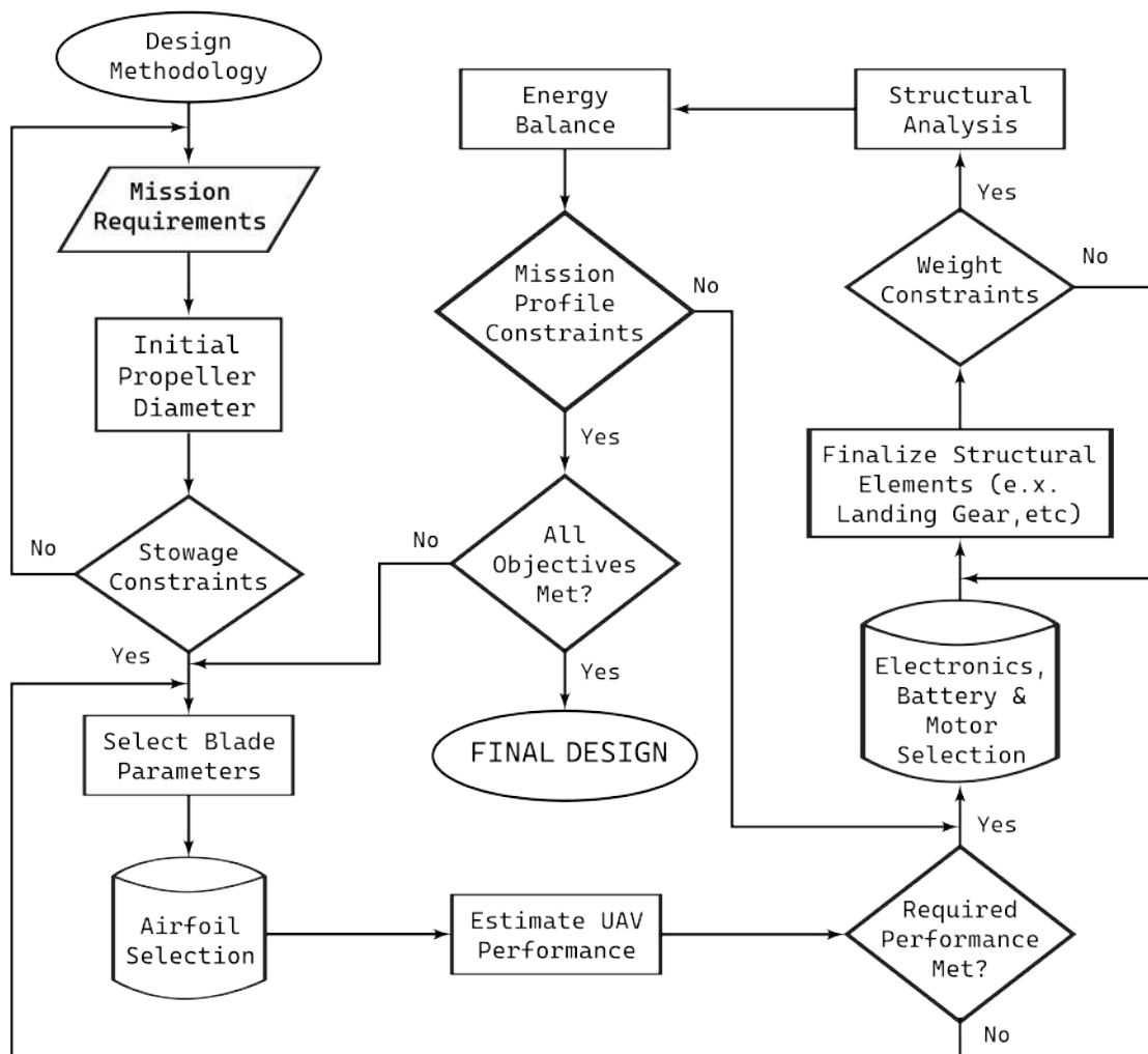
Figure 8: Design Methodology
