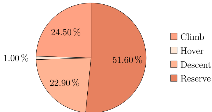
Figure 38: Energy Consumed
