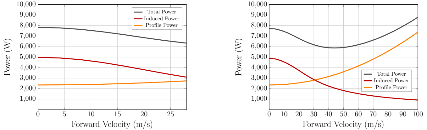
Figure 18: Variation of Total Power with Forward Velocity
