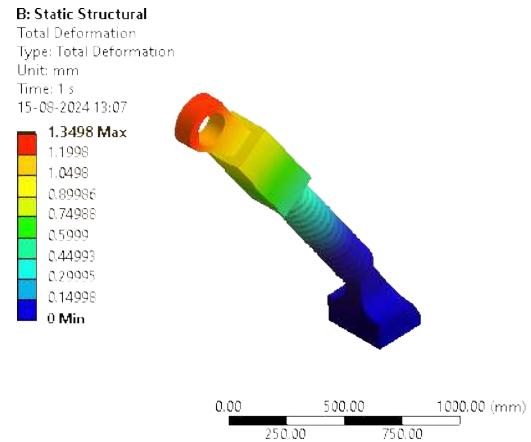
(b) Landing Gear
