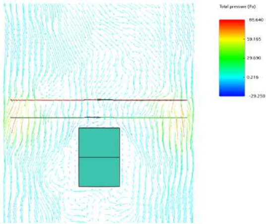
(c) Total Pressure
