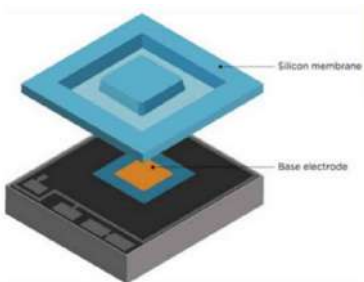
Figure 33: Pressure Sensor
