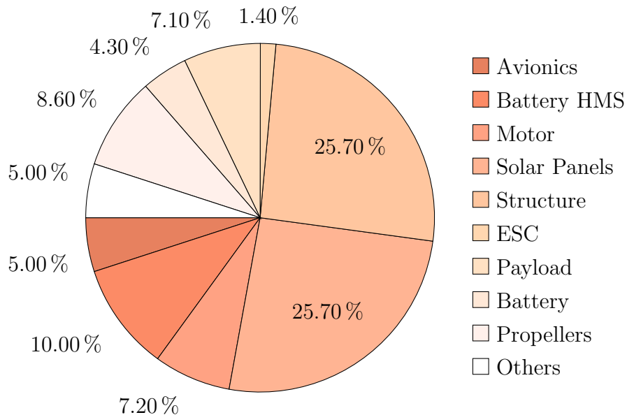
Figure 40: Mass Breakdown
