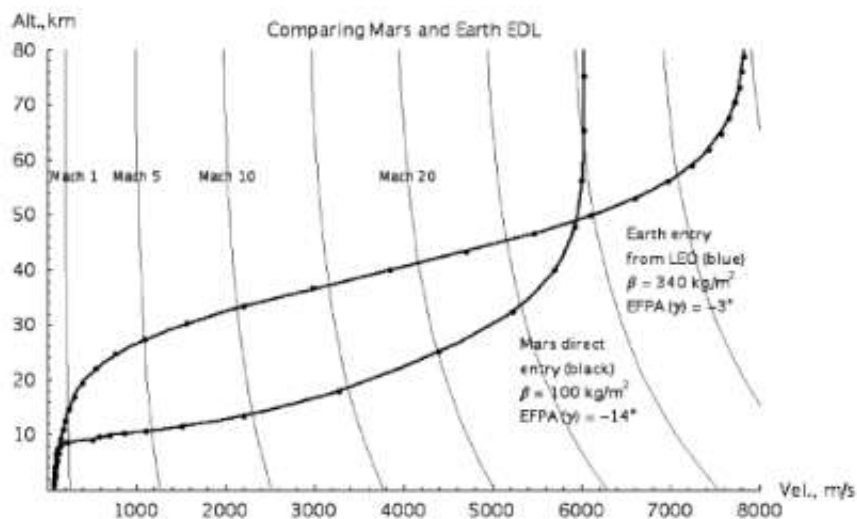
Figure 9: Altitude Velocity Map [2]
