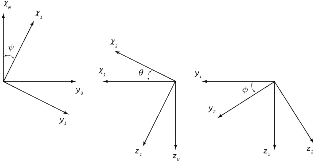
Figure 36: Pod Euler Angles
