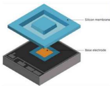
Figure 49: Pressure Sensor
