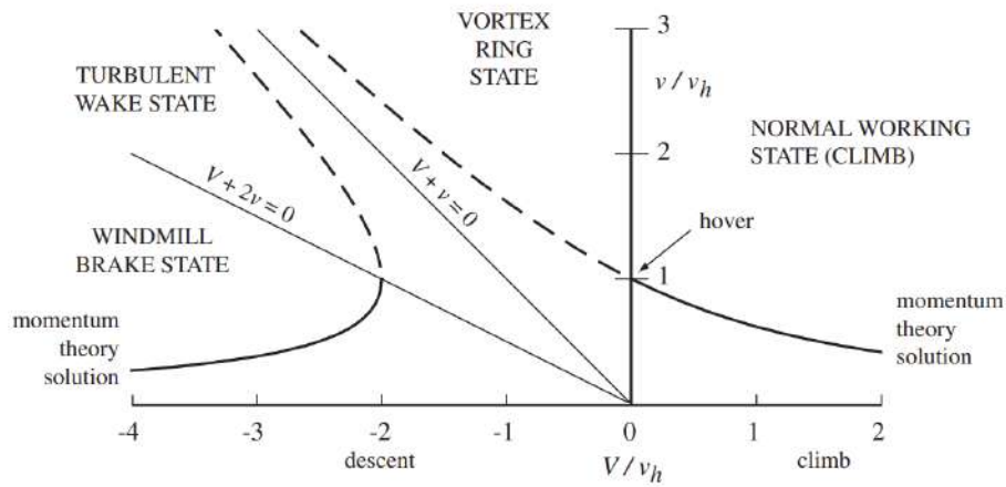
Figure 29: Momentum Theory results in Vertical Flight [3]
