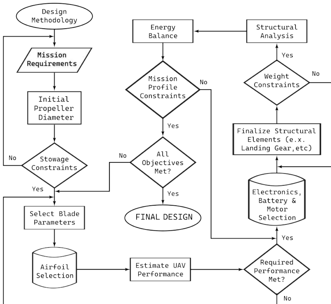
Figure 12: Design Methodology
