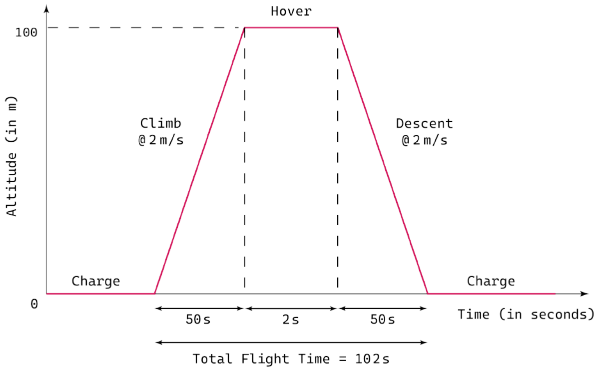
Figure 53: Mission Profile
