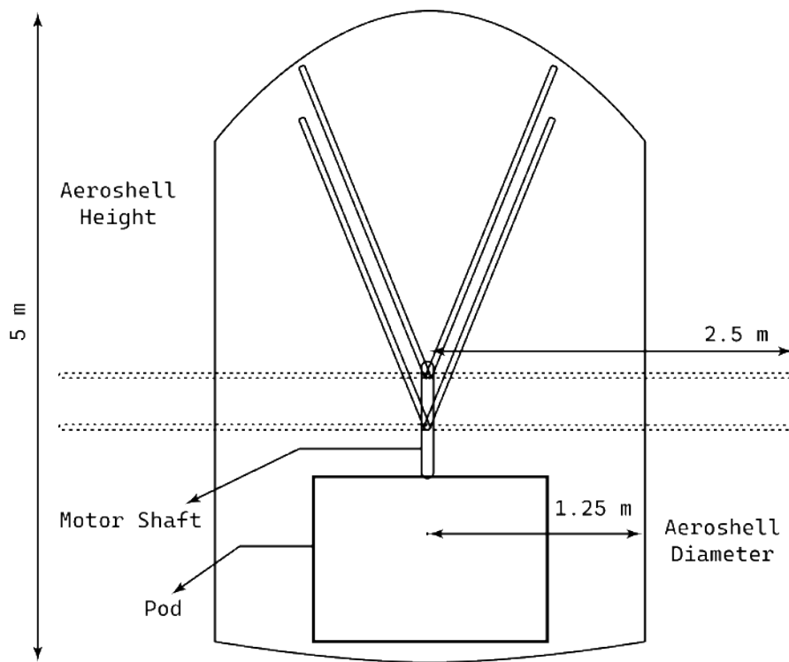
Figure 13: Proposed Stowage of the Propellers
