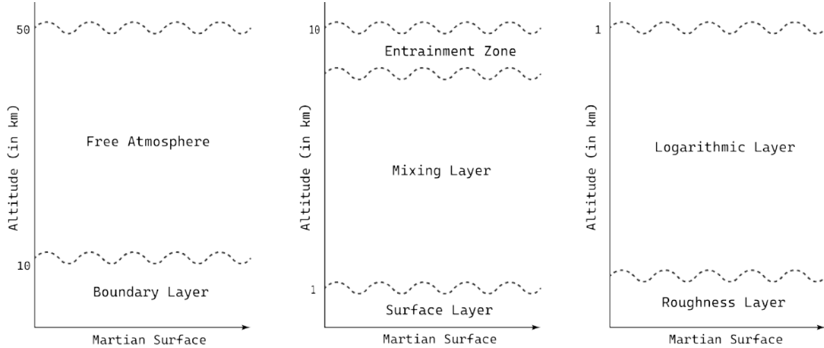
Figure 1: Martian Planetary Boundary Layer (PBL)
