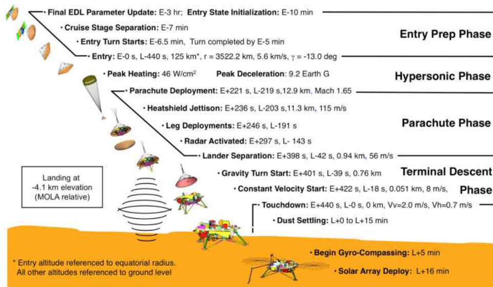
Figure 8: Actual EDL Architecture of the Phoenix Lander
