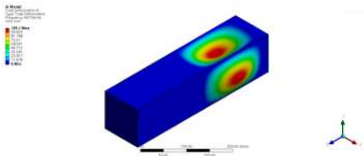
Figure 70 CubeSat Modal Analysis: Total Deformation 5
