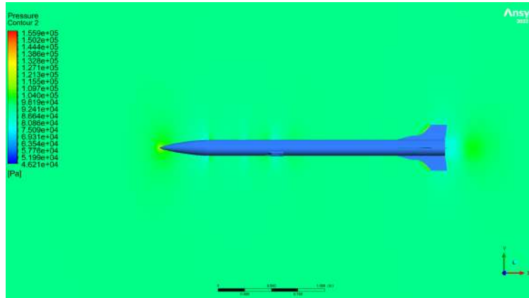
Figure 61 Pressure Contour at Mach 0.9
