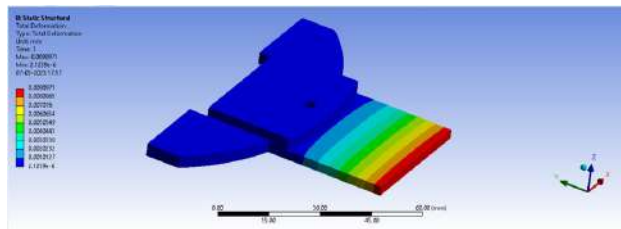
Figure 16 Ansys simulation showing of total deformation for brake plate
