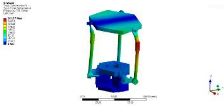
Figure 74 Stewie Modal Analysis: Total Deformation 4
