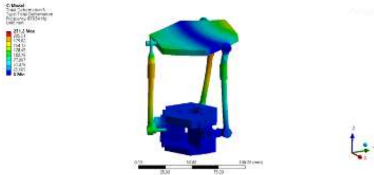
Figure 71 Stewie Modal Analysis: Total Deformation 1
