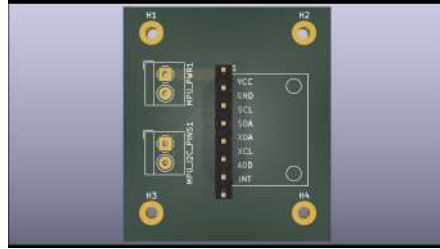
Figure 22 3D Render of Secondary Circuit Board
