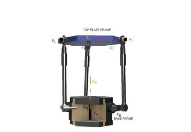
Figure 18 Representation of Reference Frames
