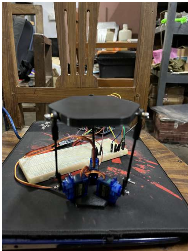
Figure 43 Payload Prototype Test
