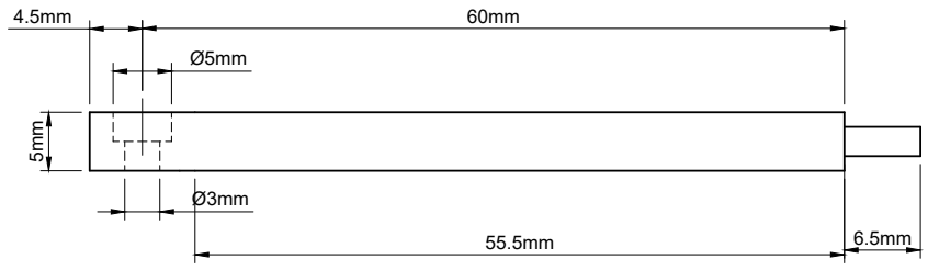
Front view (3:1)
