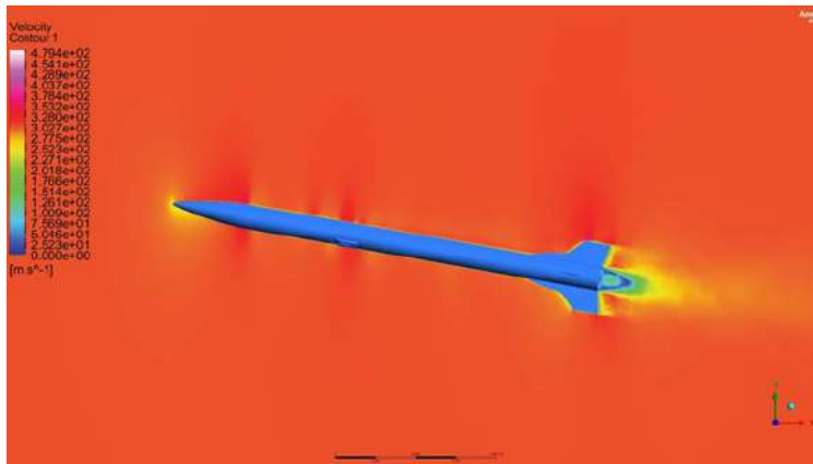
Figure 64 Velocity Contour at Mach 0.9 for 10 degree angle of attack
