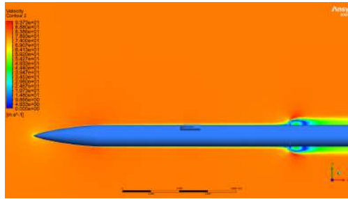
Figure 15 Velocity Contour on the Airbrakes at 80m/s
