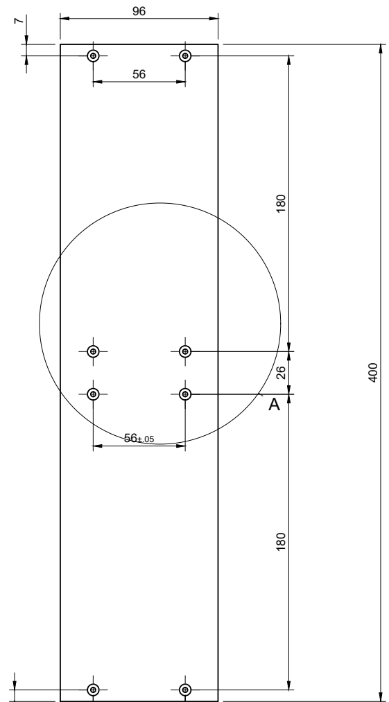
Front view (1:1.5)
