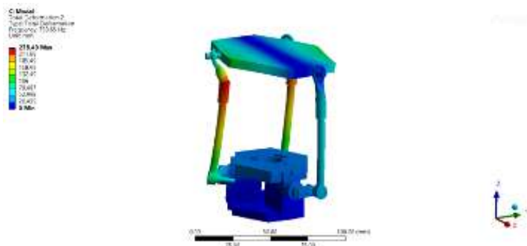
Figure 73 Stewie Modal Analysis: Total Deformation 3
