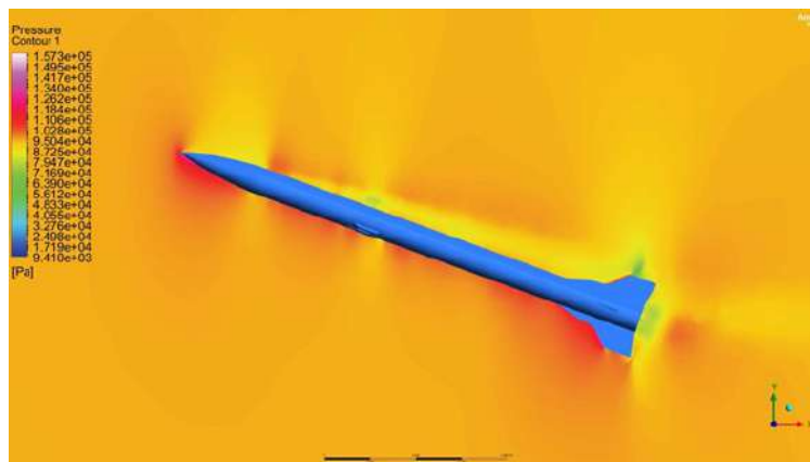
Figure 63 Pressure Contour at Mach 0.9 for 20 degree angle of attack
