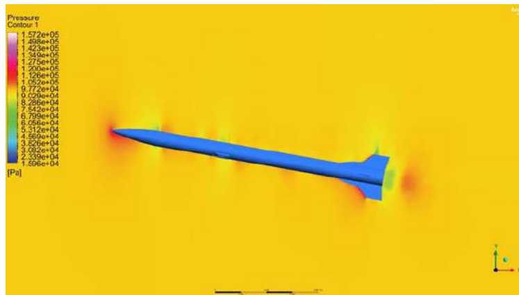
Figure 62 Pressure Contour at Mach 0.9 for 10 degree angle of attack
