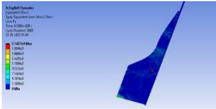
Figure 58 Explicit Dynamics Simulations Results of Fin
