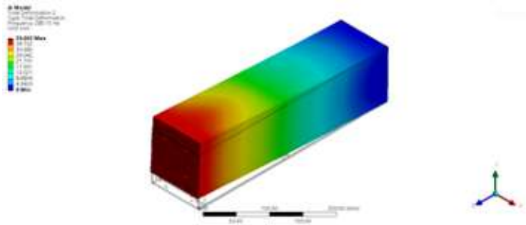
Figure 68 CubeSat Modal Analysis: Total Deformation 3
