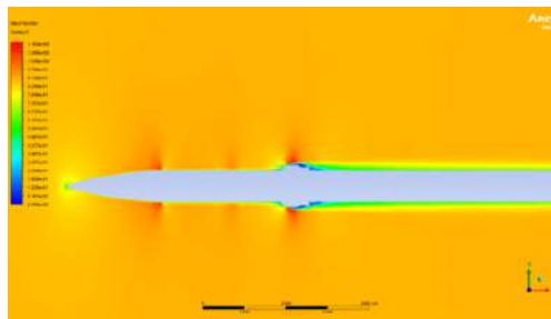
Figure 12 Velocity contour over the rocket at Mach 0.9
