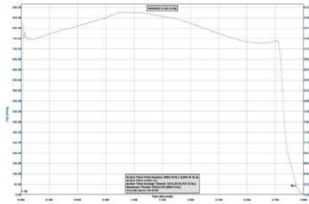
Figure 26 Thrust-Time Curve
