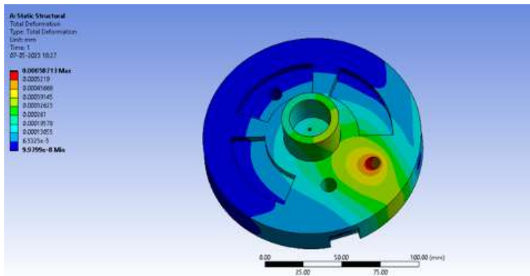
Figure 60 Recovery Bulkhead Total deformation due to force of rocket weight
