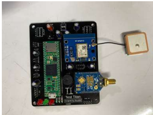
Figure 32 Ground Station PCB
