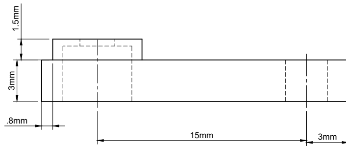
Front view (8:1)
