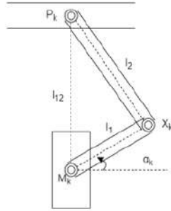
Figure 19 Side View of Leg
