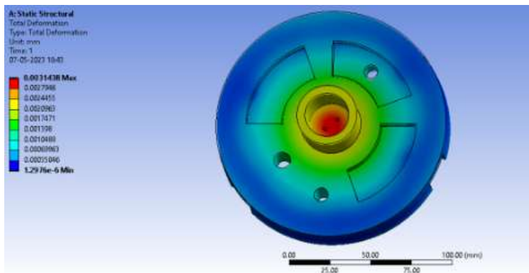
Figure 59 Recovery Bulkhead total deformation due to force of ejection charge
