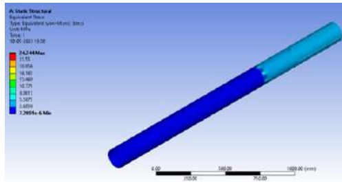
Figure 4 Von Mises Stress Profile of Body Tube Assembly under Initial Thrust Loading
