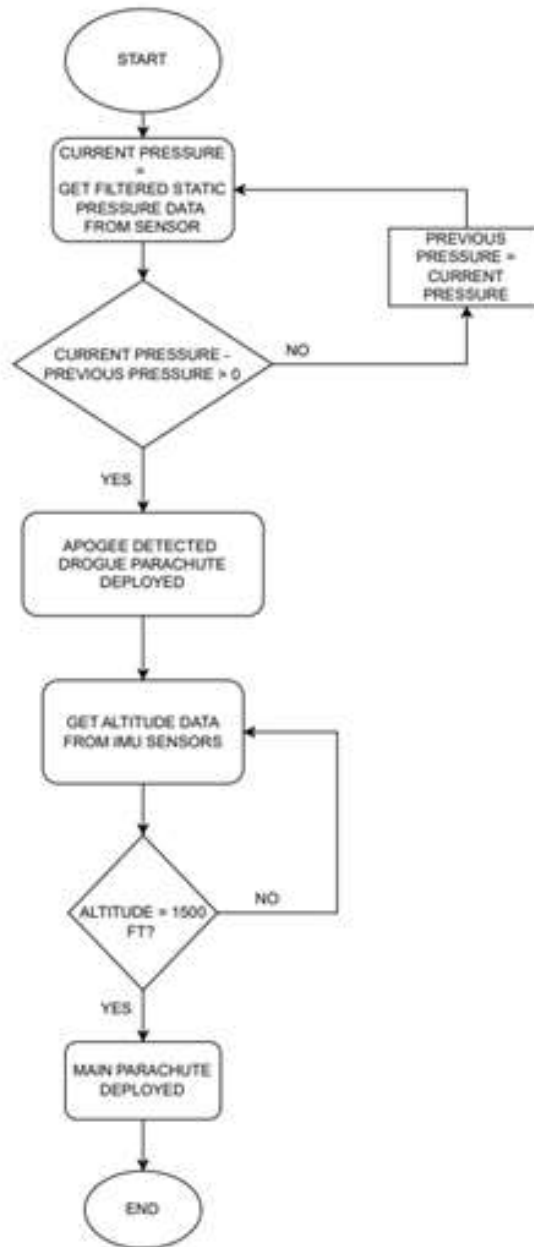
Figure 76 Flow Chart for Apogee detection and parachute deployment events
