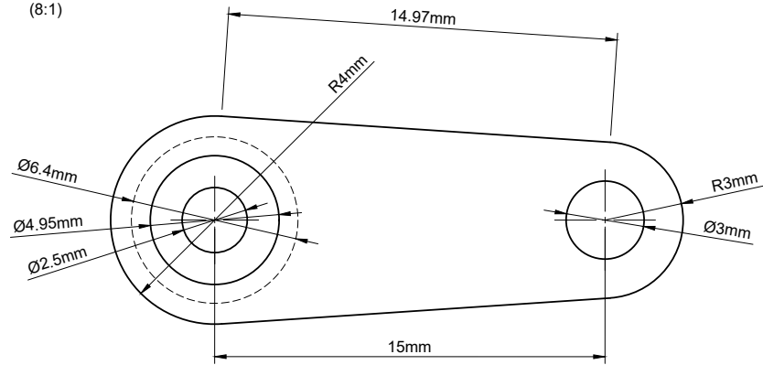
Top view (8:1)
