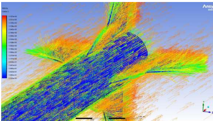
Figure 57 Velocity contour of air on the leading-edge extended fins at M 0.9
