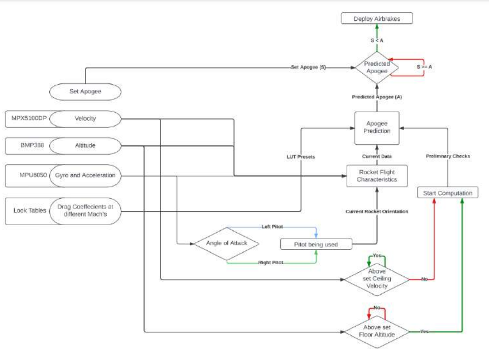
Figure 30 Flow Chart for Air Brakes Control System
