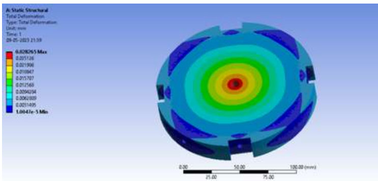
Figure 55 Thrust Plate Simulation
