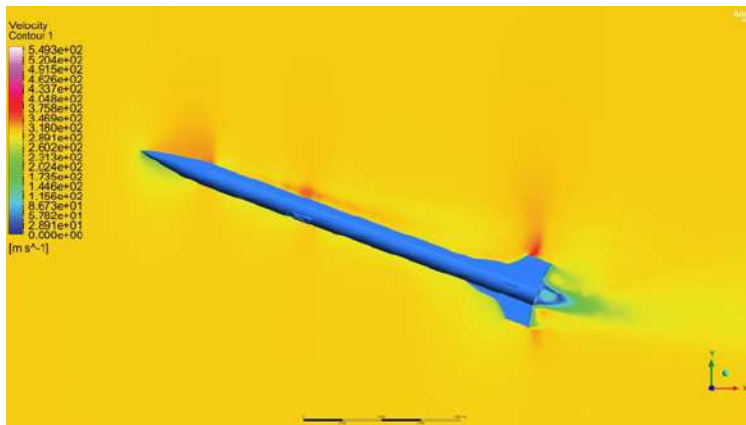
Figure 65 Velocity Contour at Mach 0.9 for 20 degree angle of attack
