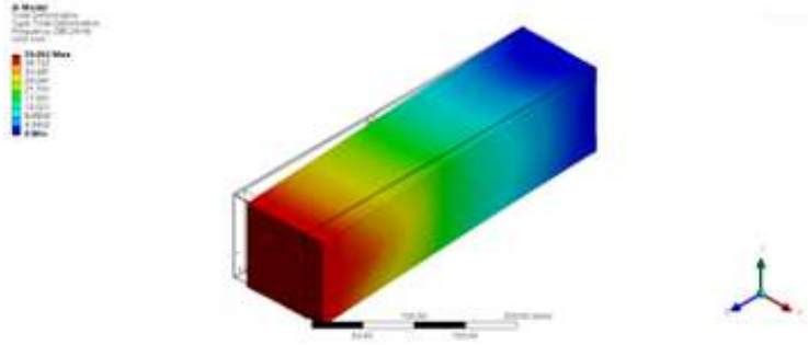
Figure 67 CubeSat Modal Analysis: Total Deformation 2
