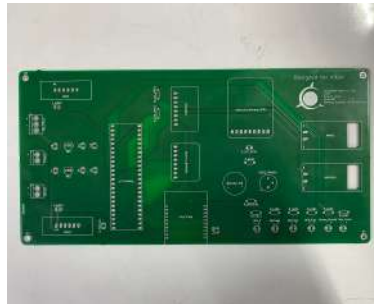
Figure 28 Actual SRAD Primary Flight Computer
