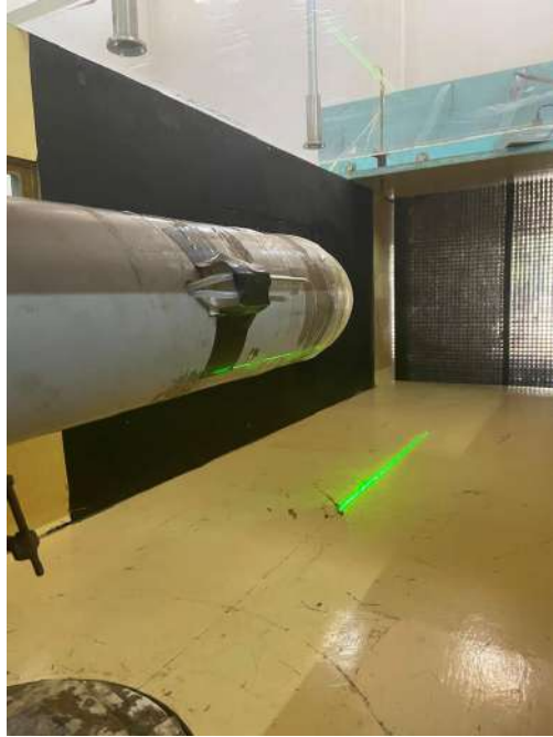
Figure 35 Pitot Testing
