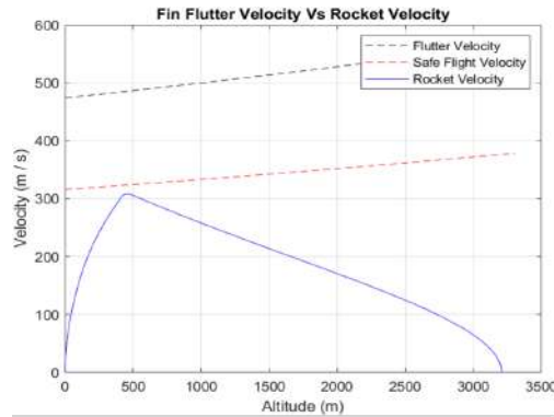
Figure 10 Fin Flutter Velocity vs. Rocket Velocity
