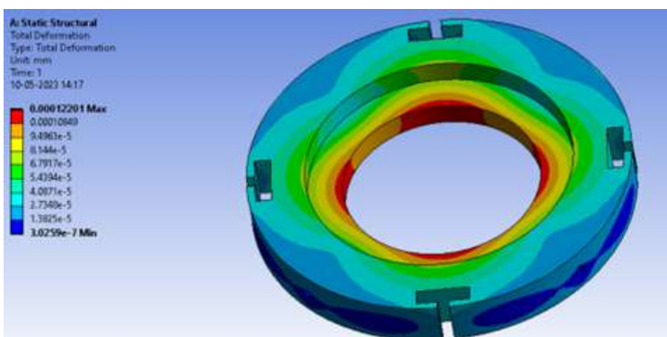
Figure 56 Retainer Simulation
